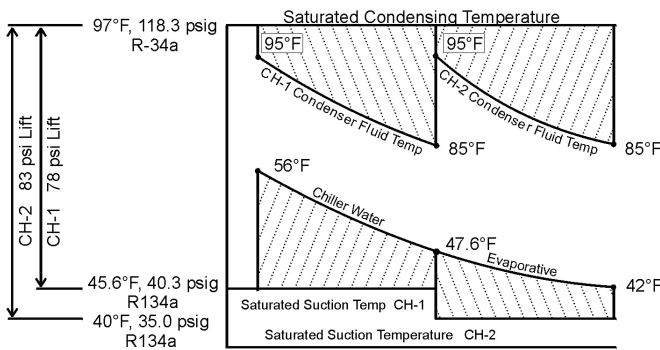
Figure 13: Series Counterflow Flow
