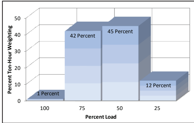
Figure 16: IPLV Defined by AHRI Standard 550/590
