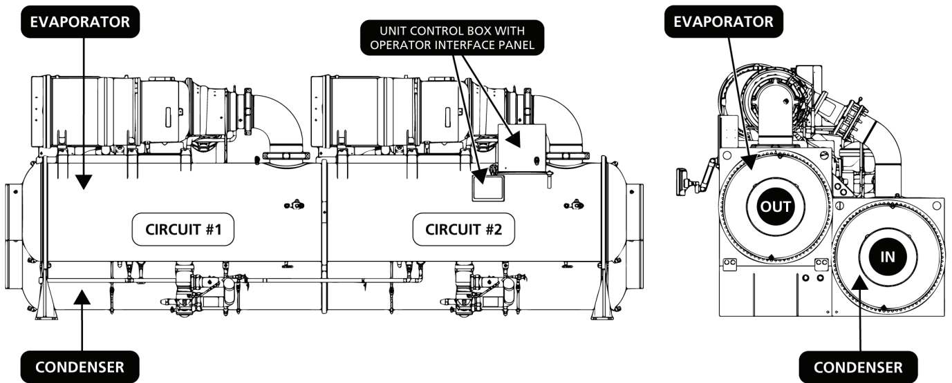
Figure 9: WCC Layout
