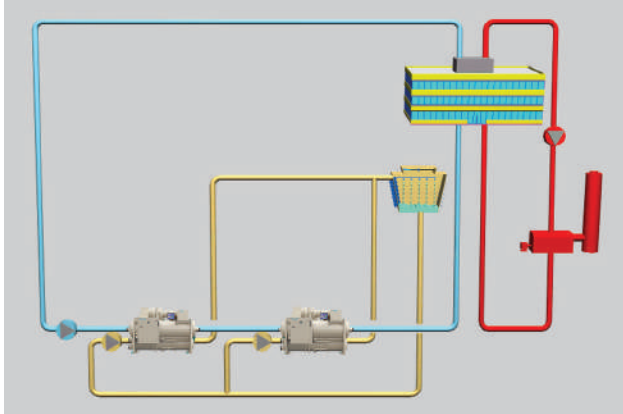
Figure 12: Series Parallel Flow
